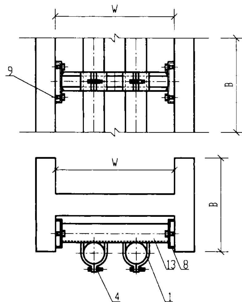
III沿钢柱支架敷设
