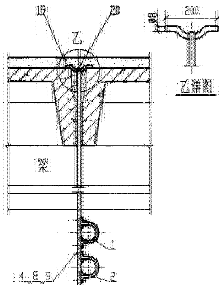
IV 沿预制板缝在梁下吊杆敷设
