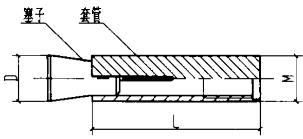
H型外迫式内牙胀锚螺栓
