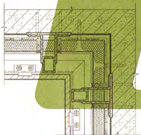
③ 幕墙阴角
