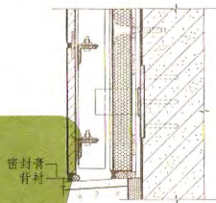
⑤ 勒脚
