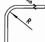
d \leq 25 \quad R \geq 4d (6d) d > 25 \quad R \geq 6d (8d) (括号内用于顶层边节点)
