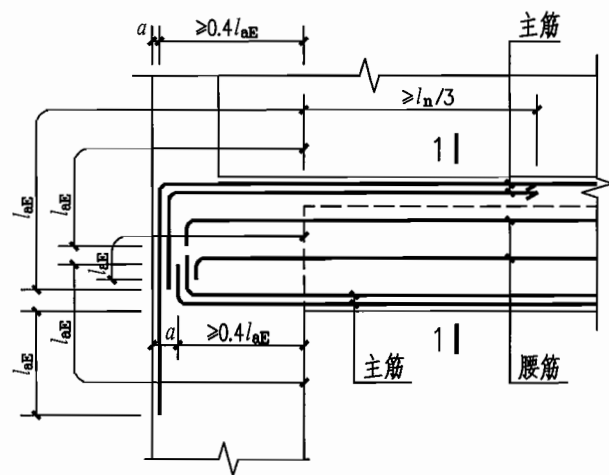
框支梁主筋和腰筋的锚固
