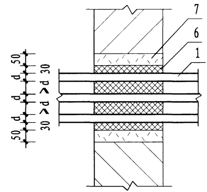
II 速固型堵料封堵
