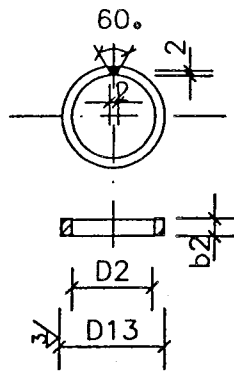
② 翼环
