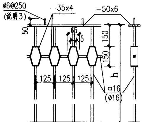
Ⓕ 方钢 Ⓖ 圆钢
