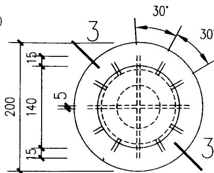
(c) 铸铁罩
