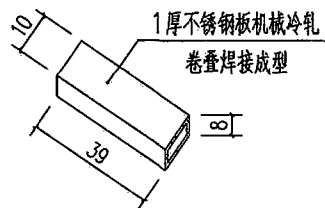
A 竖向边框加强肋
