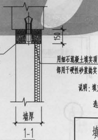
③ (墙体顶部锚栓加钢筋大样)
